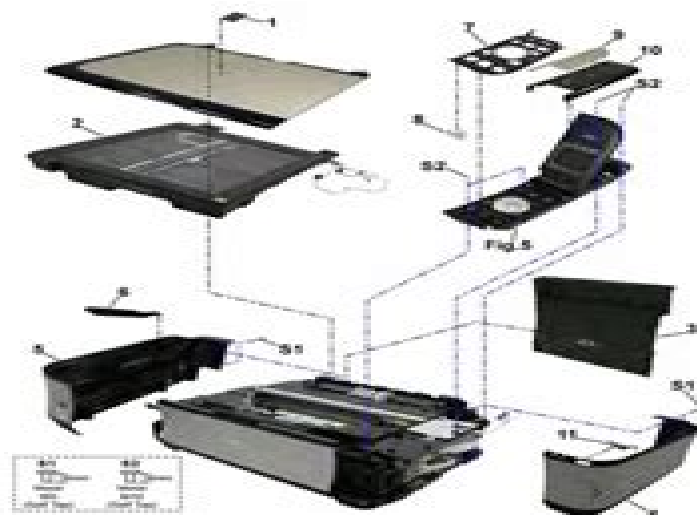
EXTERNAL COVERS & SCANNER UNIT
