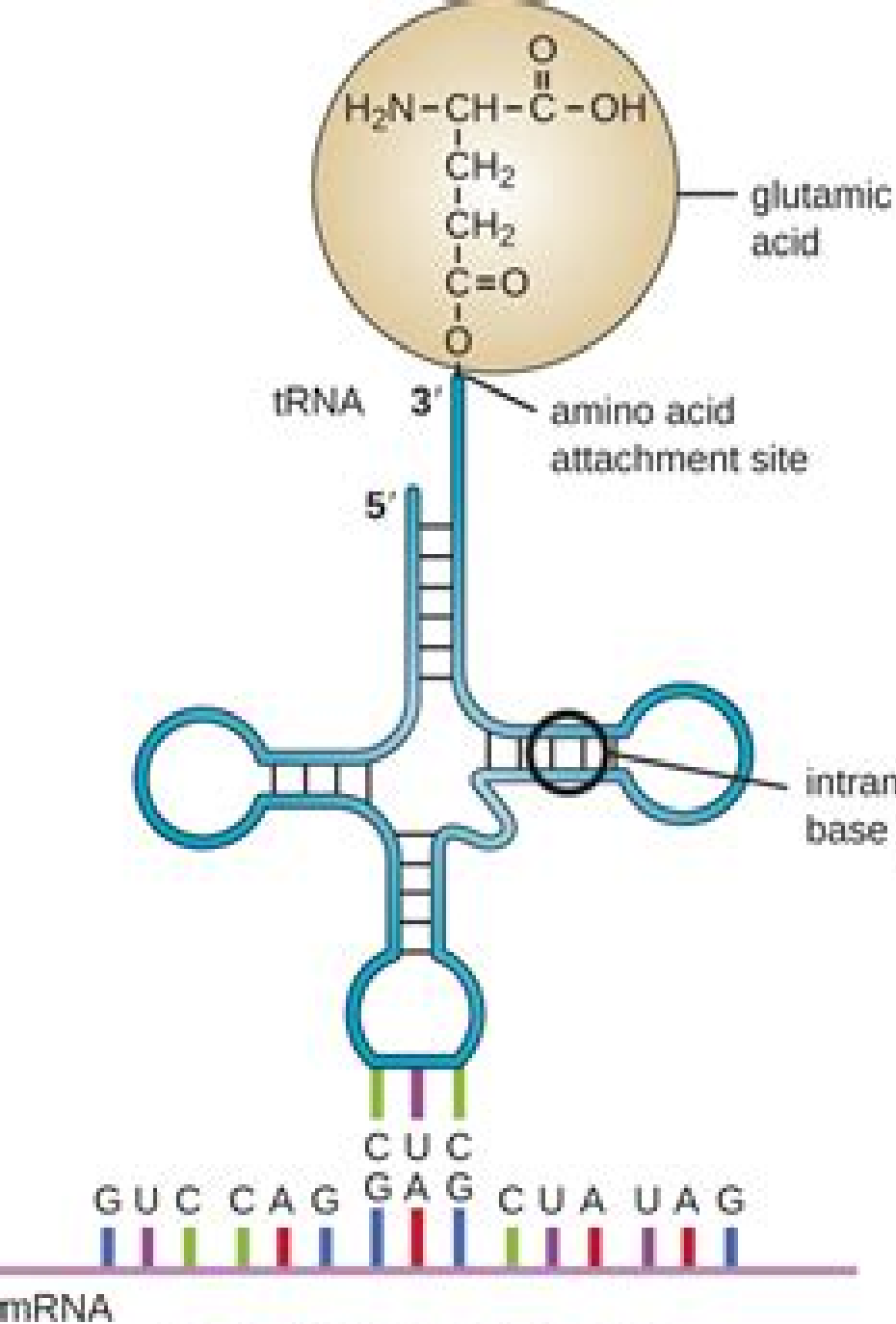
tRNA 2-dimensional structure
