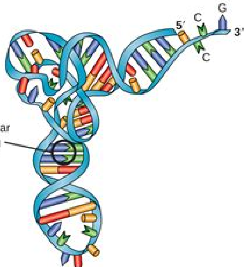
tRNA 3-dimensional structure
