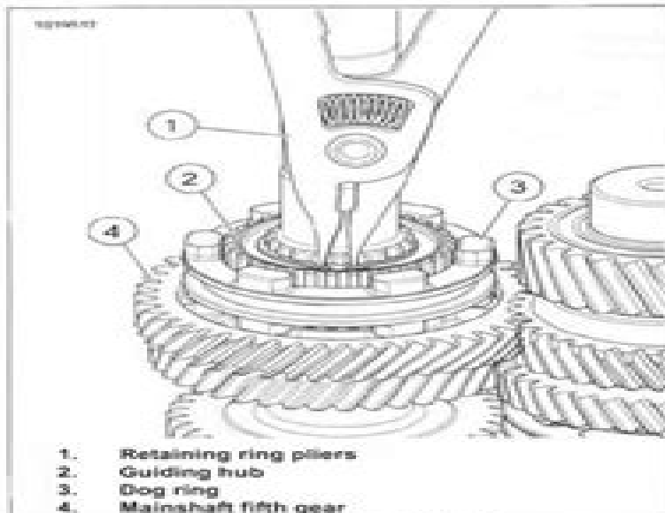
Figure 5-50. Mainshaft Fifth Gear
