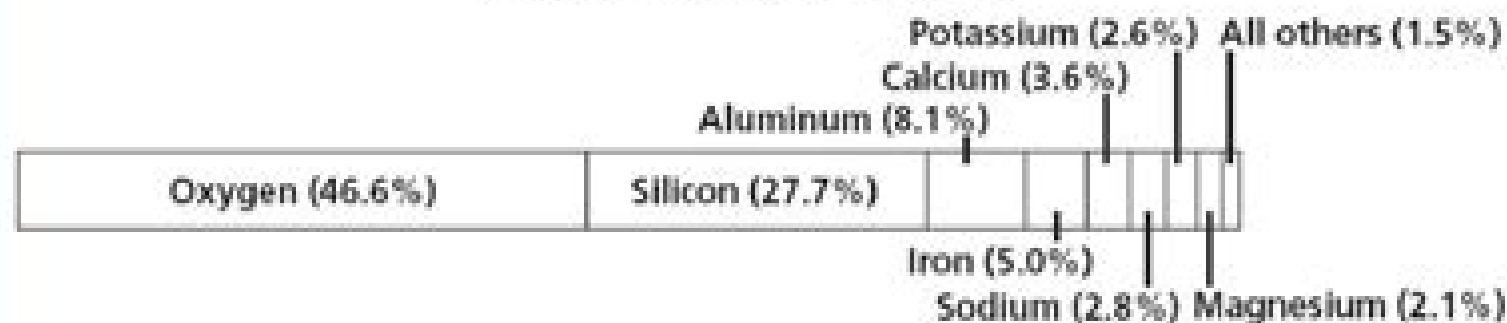
Elements in Earth's Crust
