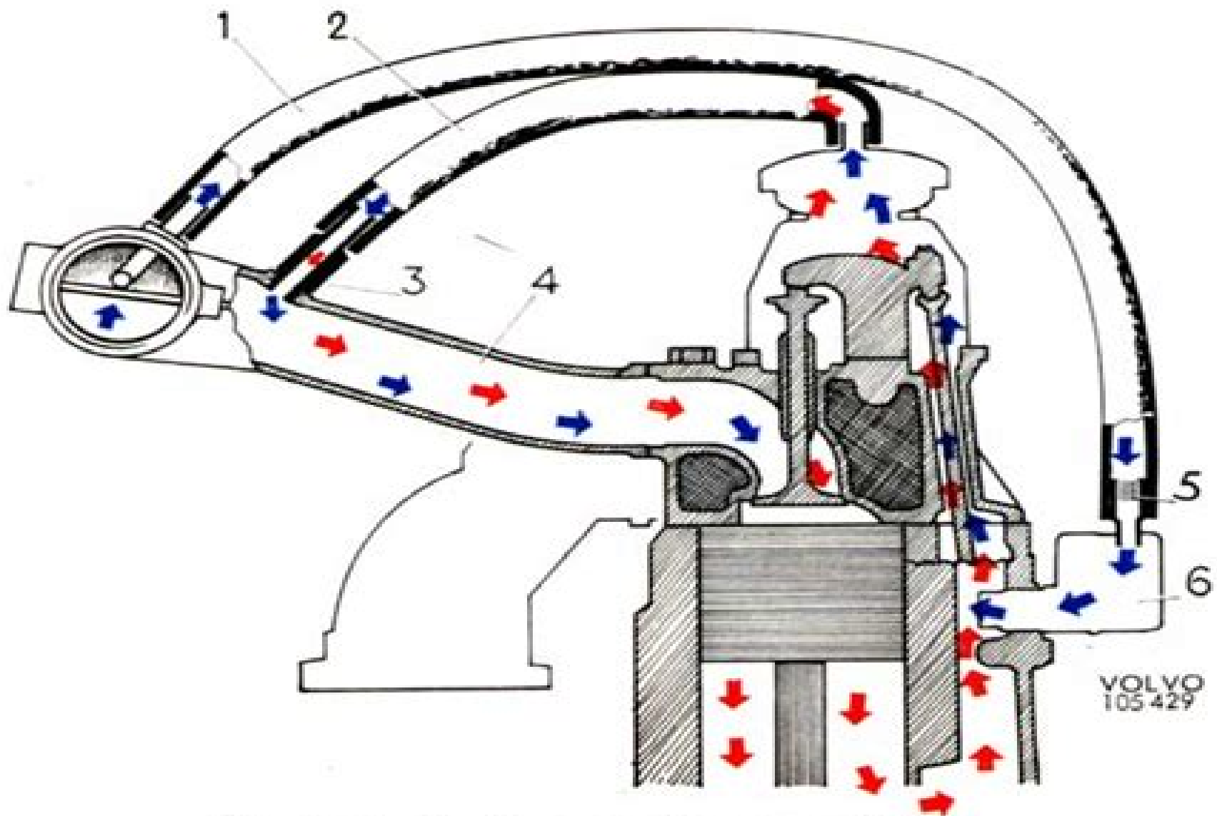
Fig. 2-12. Positive crankcase ventilation
