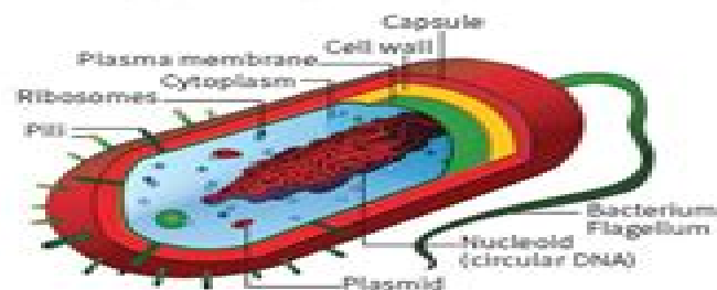
Figure 1.3 Prokaryotic cell
