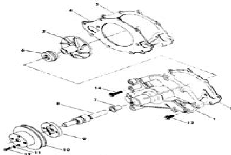
Fig. 42 — Circulating Pump
