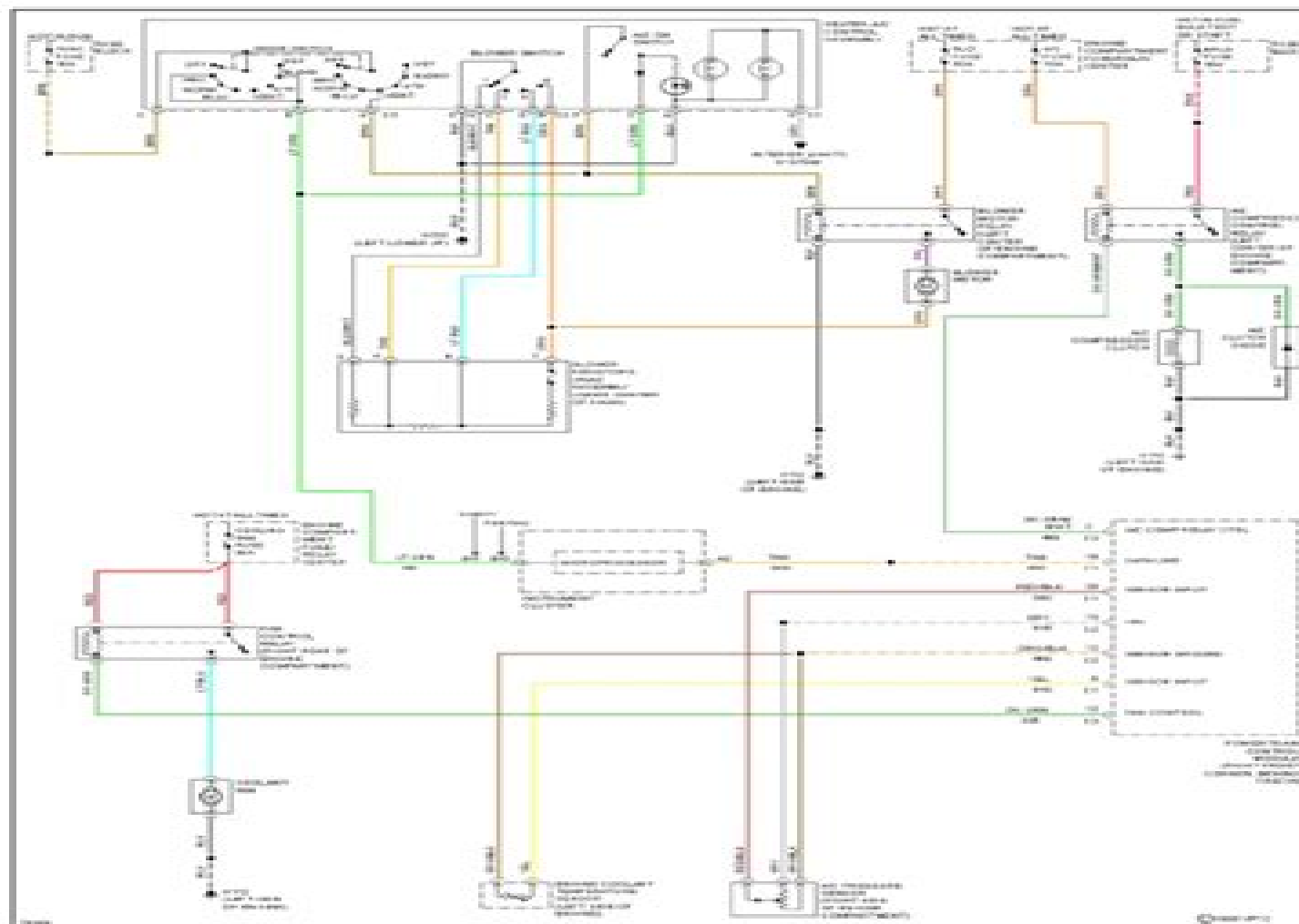
Fig. 1: A/C Circuit
