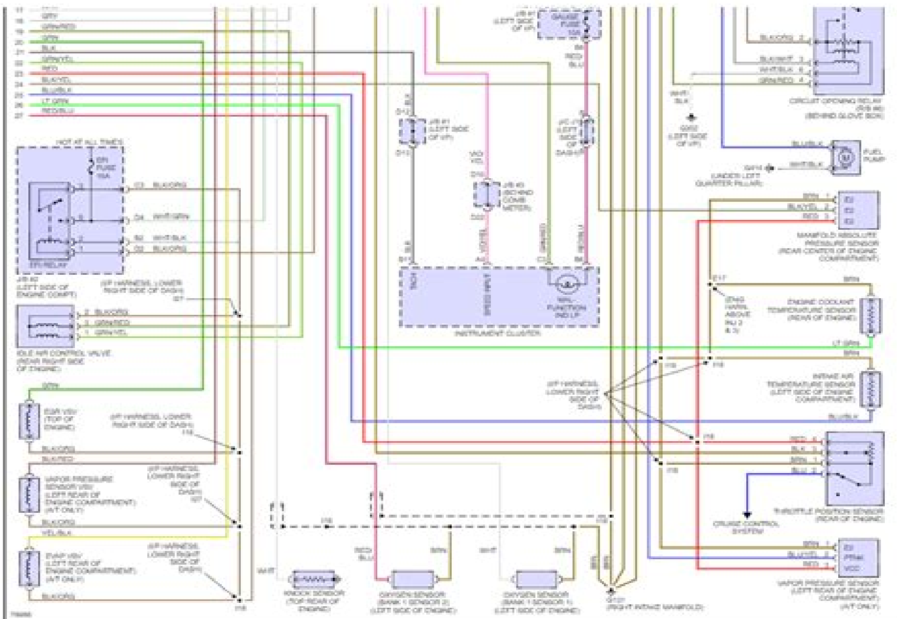
Fig 2: 2.2L, Engine Performance Circuits (2 of 2)
