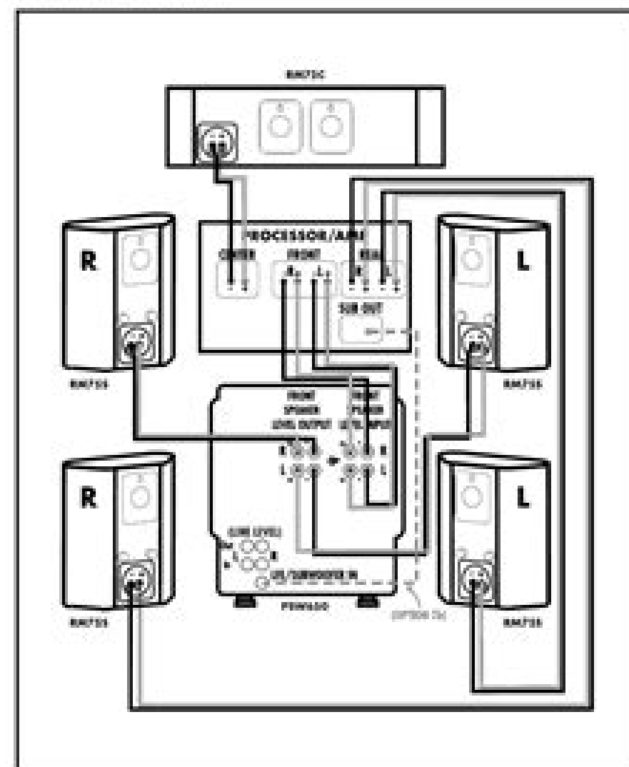
Figure 2: Dolby Digital 5.1 System (1 or 2 Ch, Page 4-5)
