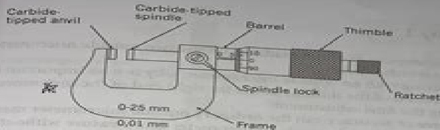
Figure 4.1: Outside micrometer
