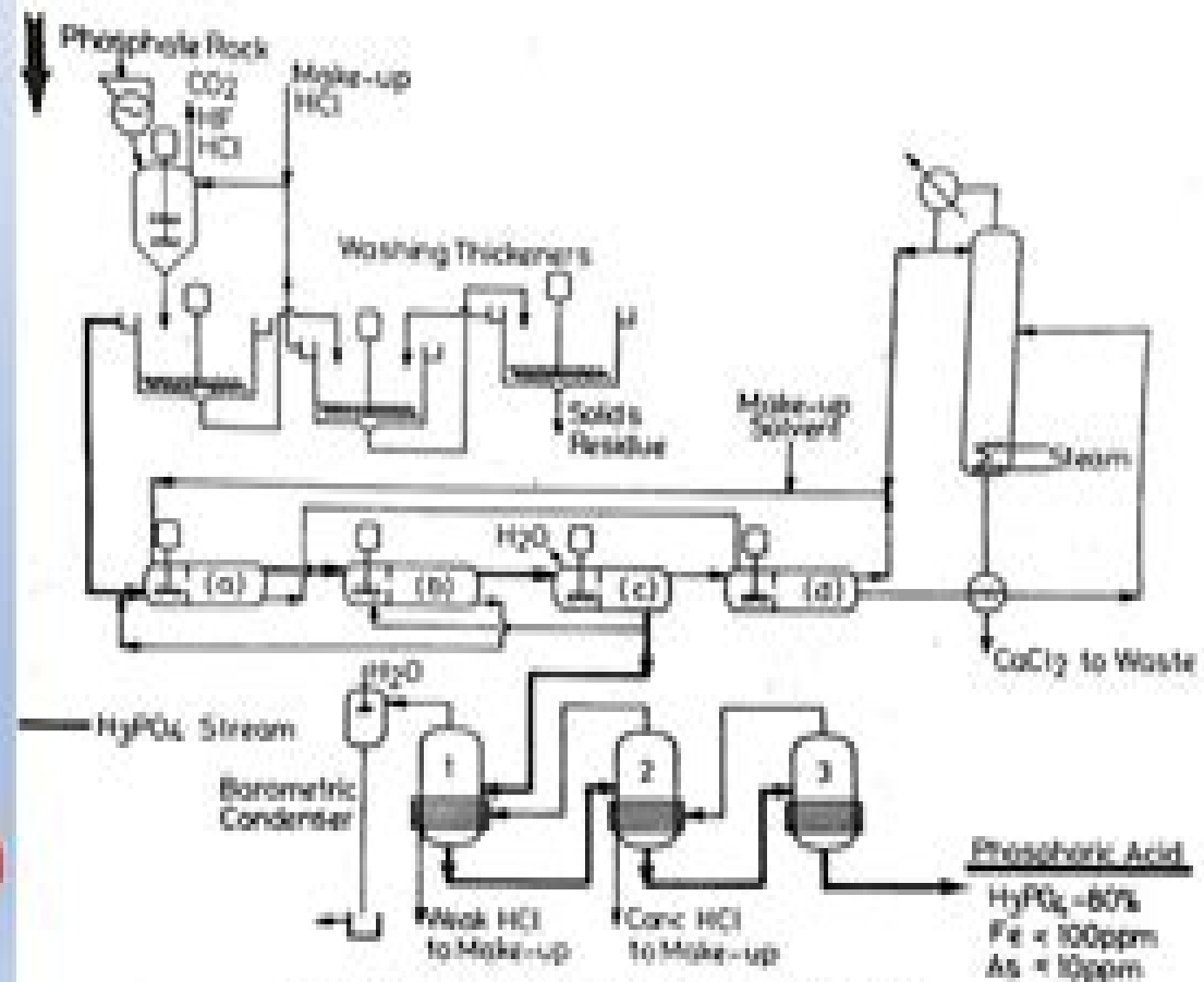
Fig. 1P-3. Production of phosphoric acid by HCl leaching.
