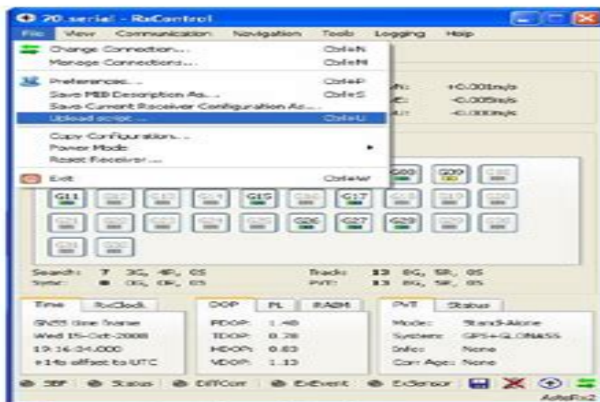
Figure 10: Upload Script
