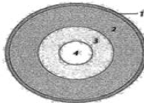
Earth's layers
