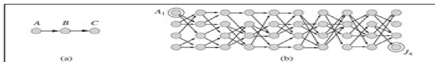
Figure 9.9 (a) Finding a path from A to C can lead Prolog into an infinite loop. (b) A
