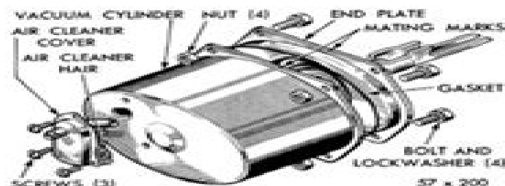
Fig. 23 — Removal of Air Cleaner and Vacuum Cylinder)
