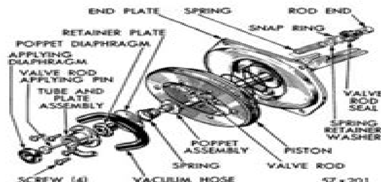
Fig. 24 — Disassembly of Tube and Plate Assembly
