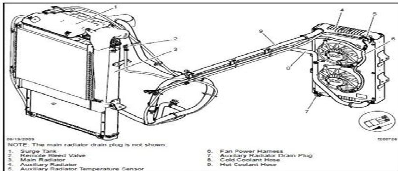
Fig. 3. Coolant System, Argosy, with Auxiliary Radiator
