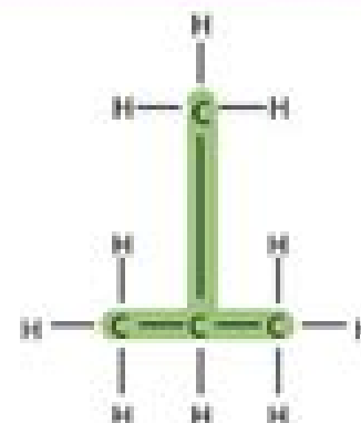
Branched carbon chain
