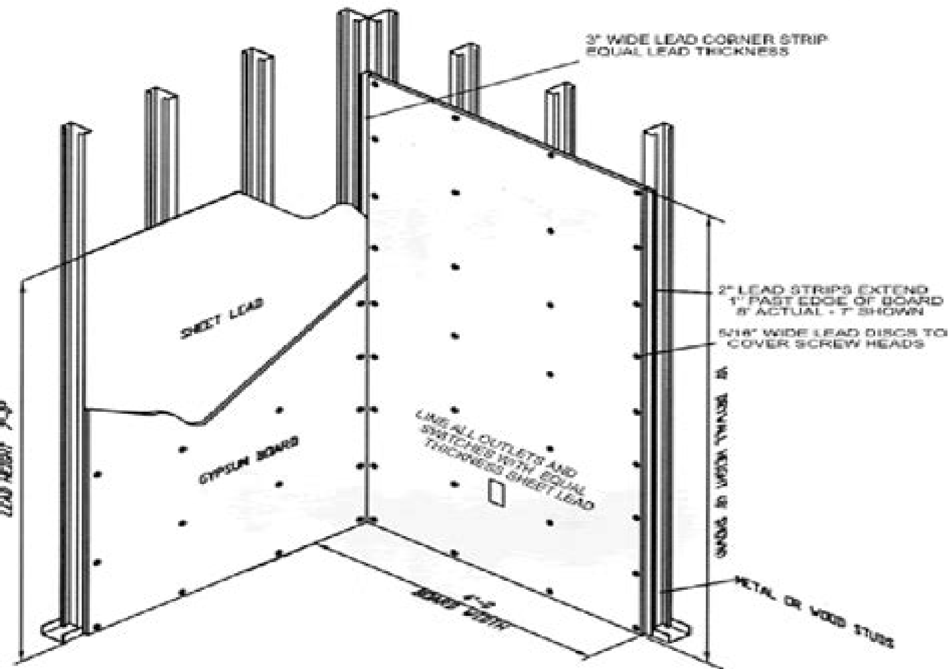
Fig. 1 A typical gypsum board wall assembly
