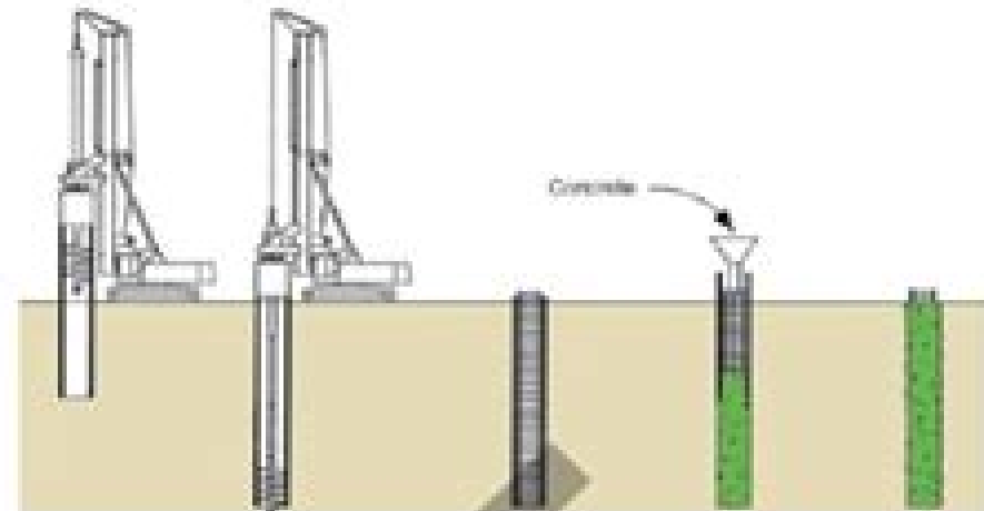
Figure 3. Standard pile construction process [4].
