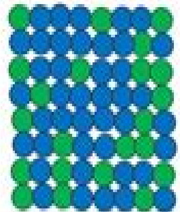
Solid solution
