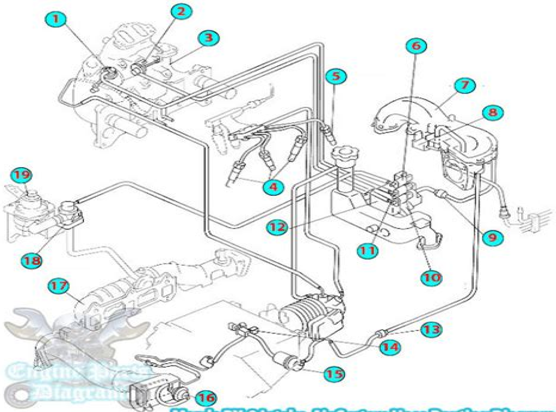
Mazda RX-8 Intake-Air System Hose Routing Diagram
