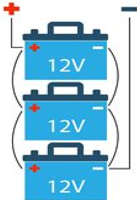
3 Parallel (Remains 12 Volt)
