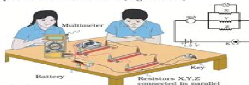
Fig.10.10.5 Circuit arrangement to show the potential difference and current in a parallel combination of resistors
