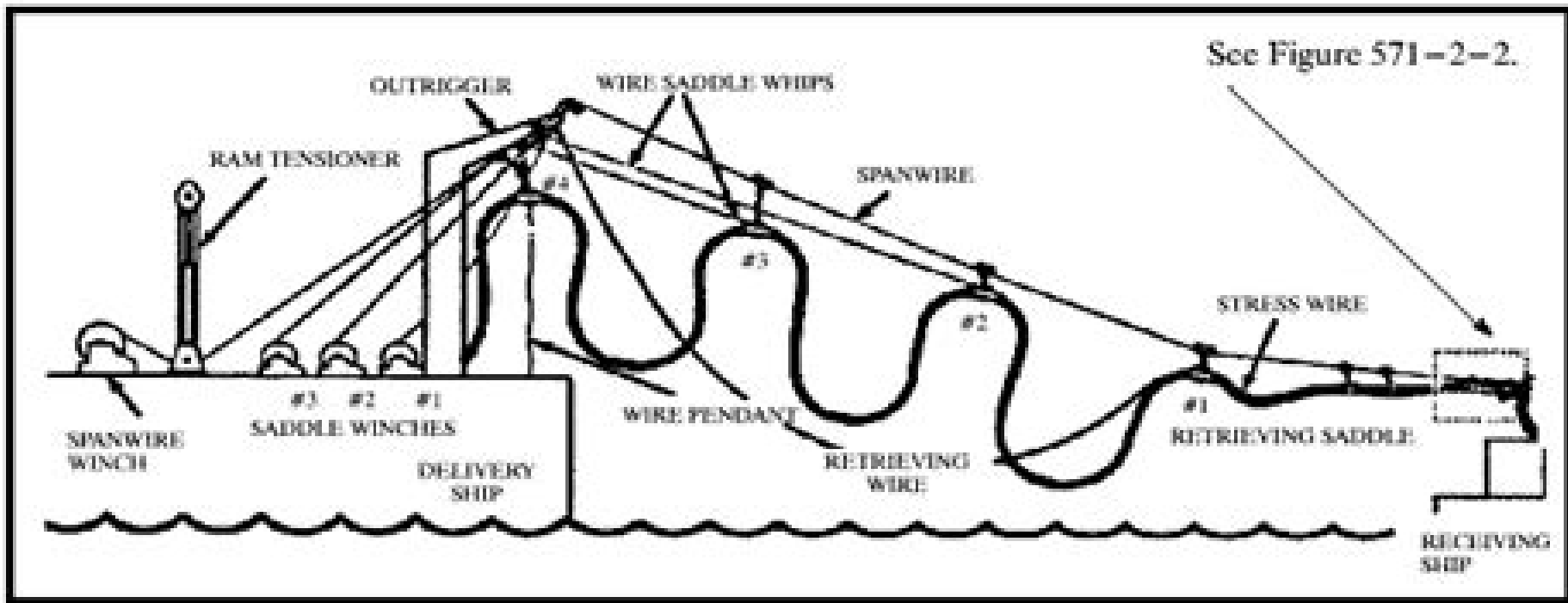
Figure 571-2-1. Fuel STREAM Rig - Single Hose with Probe
