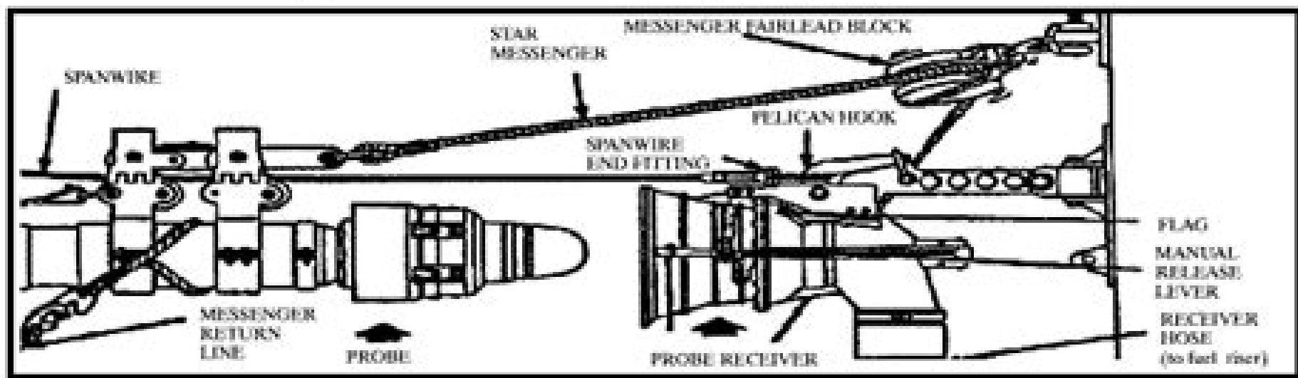
Figure 571-2-2. Single Hose Fuel STREAM Rig with Probe
