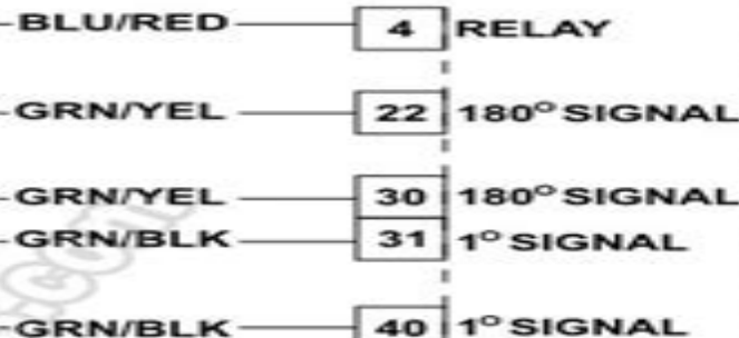
CRANK ANGLE SENSOR CONNECTOR ON DISTRIBUTOR
