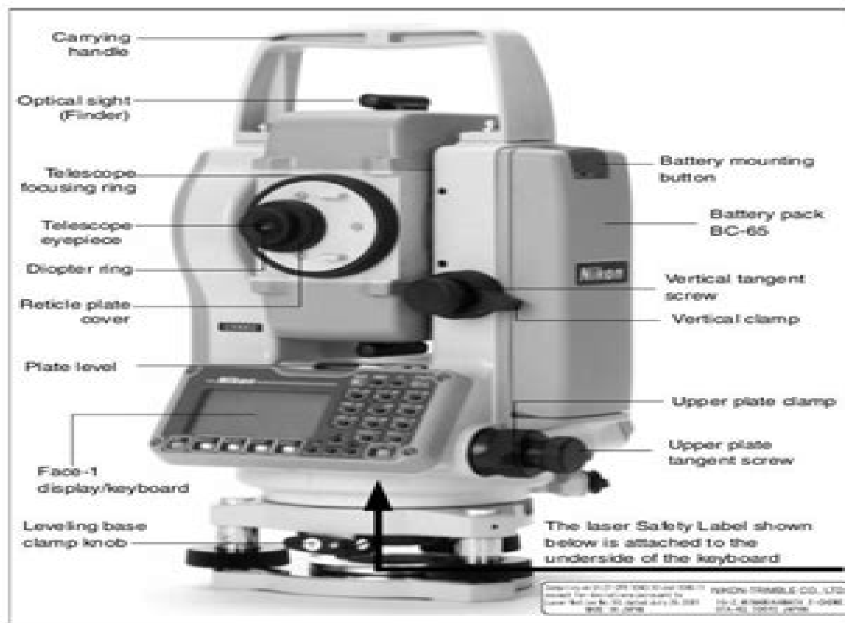
Figure 1.1 Pulse Laser Station NPL-302 series – Face-1
