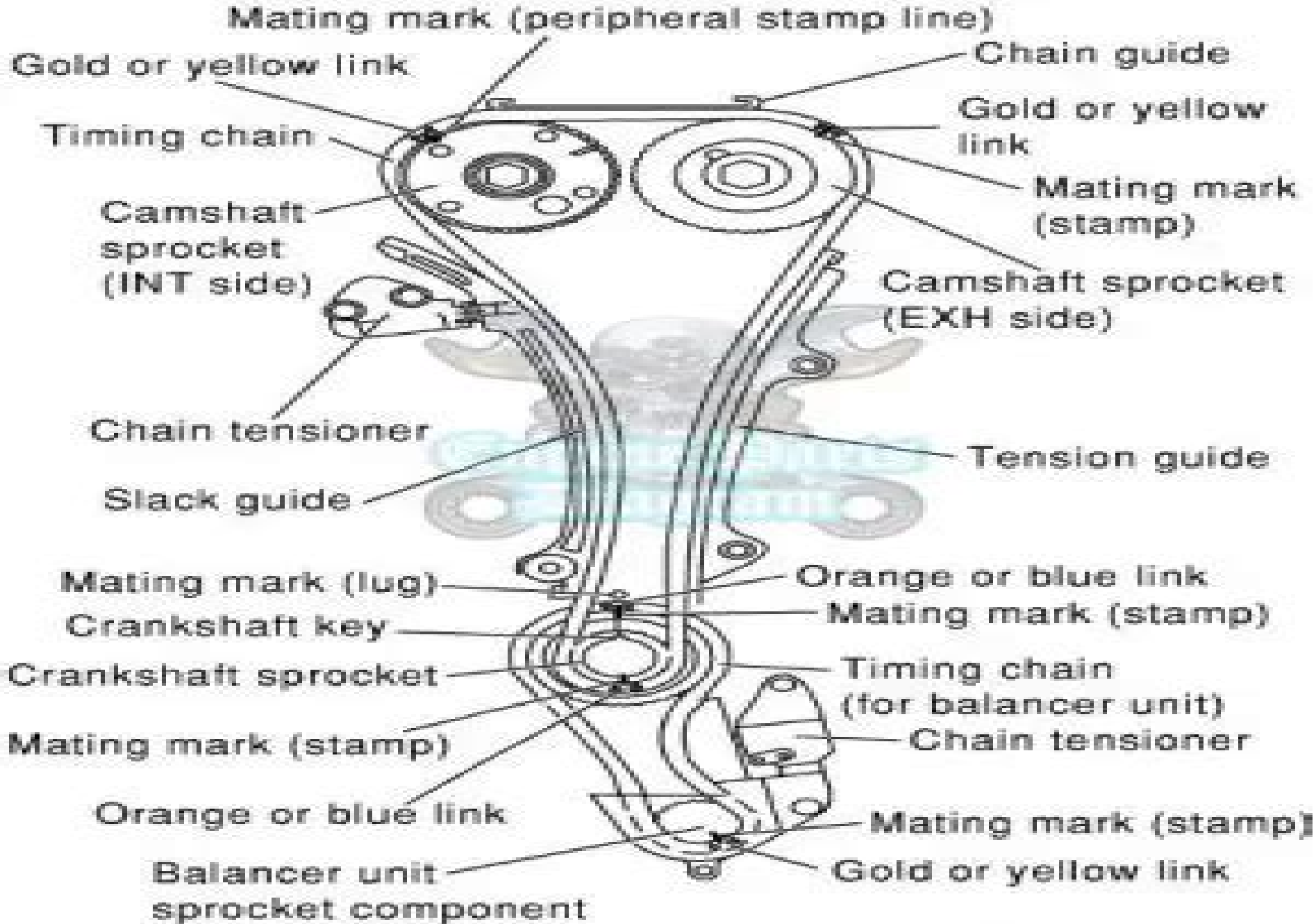
QR25DE Engine Timing Mark Diagram
