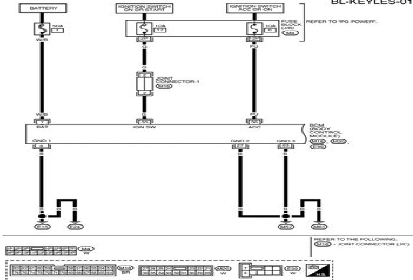
Wiring Diagram — KEYLES— FIG. 1
