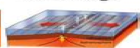
Ocean Ridge
