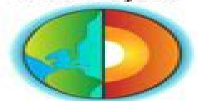
Earth Layers
