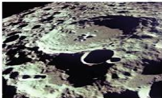
Fig. 17.7 : Surface of the moon
