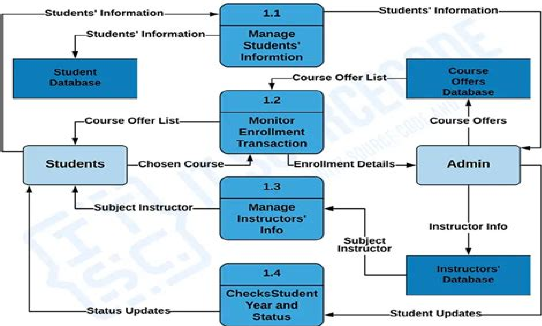
DATA FLOW DIAGRAM LEVEL 2
