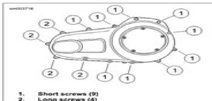
Figure 7-1. Primary Chaincase Cover Screws
