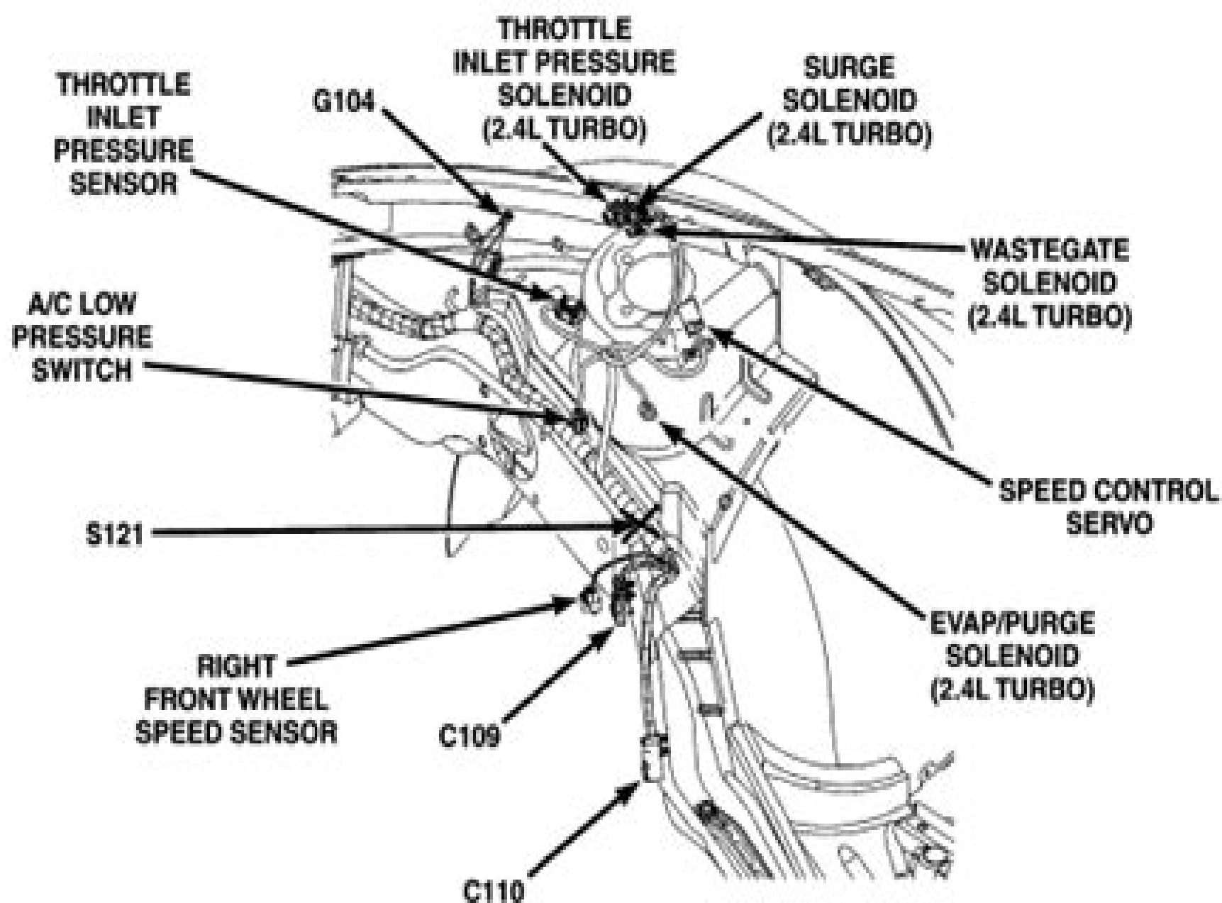
RIGHT REAR ENGINE COMPARTMENT (2.4L)
