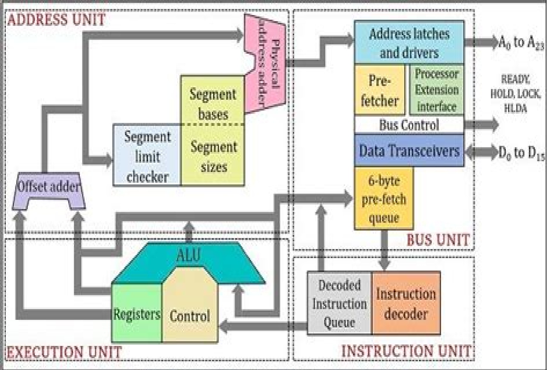
Block Diagram of 80286 Microprocessor
