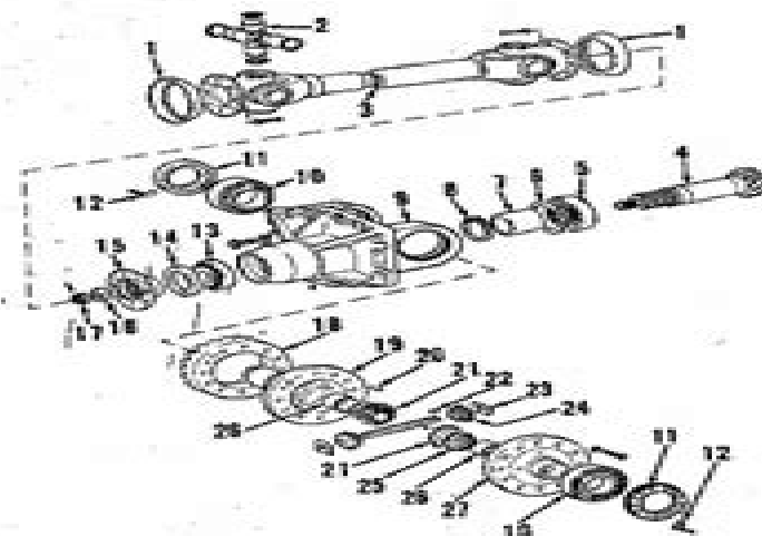
Fig. 12—Exploded view of final drive differential and drive shaft used in Model 1210 four wheel drive tractor.
