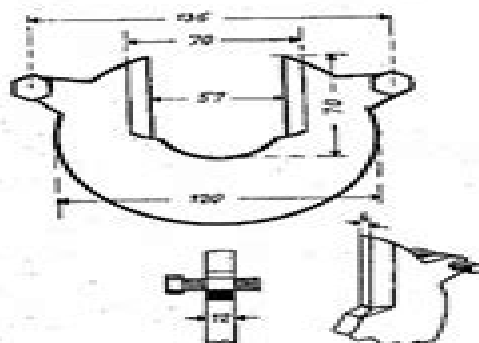
Fig. 11—A holding clamp can be fabricated locally to prevent axle movement during assembly. Dimensions are in millimeters.
