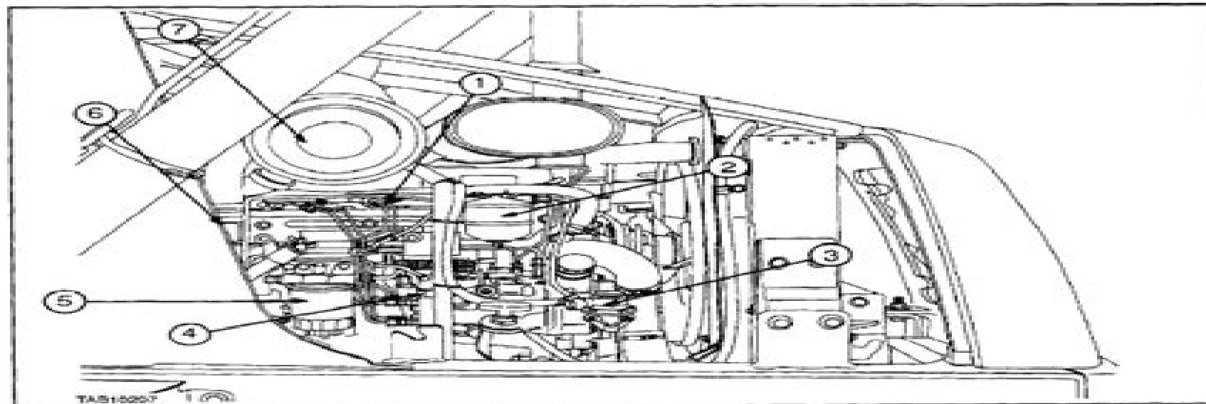
Right-Hand View of Engine
