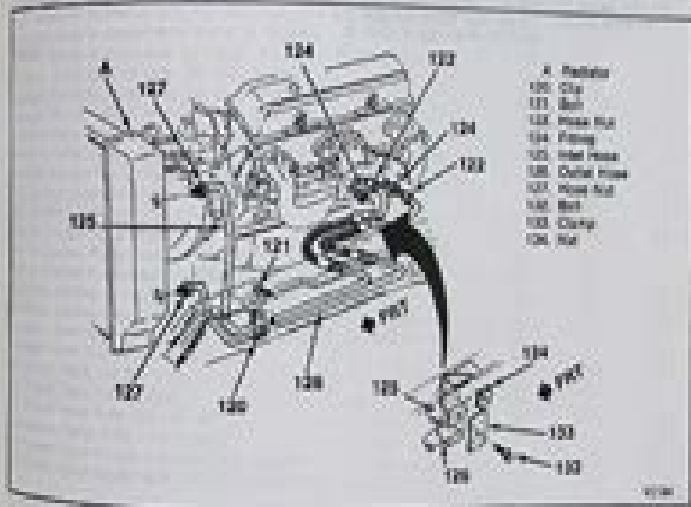
Figure 41—Engine Oil Cooler Lines (S.B. Engine)
