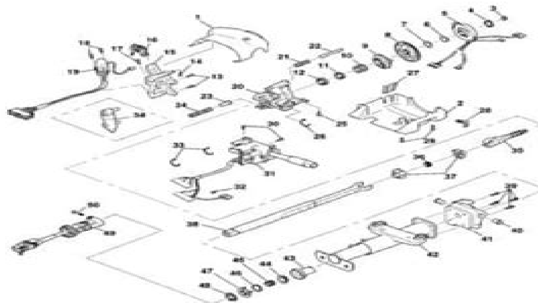
Fig. 1: Tilt Steering Column Disassembled View, Floor Shift Courtesy of GENERAL MOTORS CORP.
