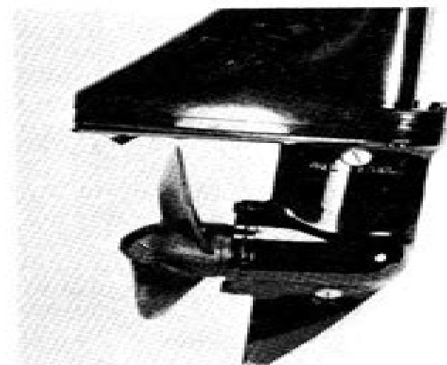
"OIL LEVEL" and "OIL" are cast into the lower unit housing near the two openings. Both screws are removed and lubricant added through the lower opening.
