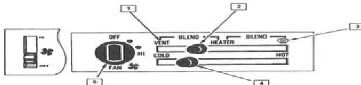
Fig. 4 Heater Ventilation System - Typical
