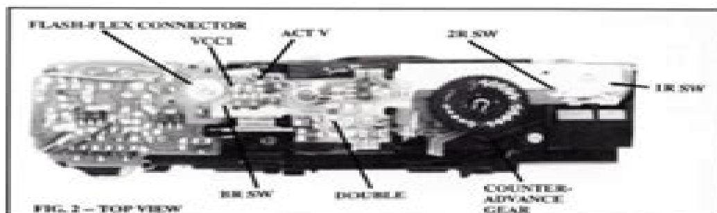
FIG. 2 -- TOP VIEW
