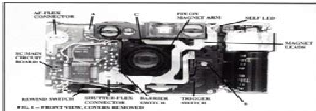
FIG. 1 -- FRONT VIEW, COVERS REMOVED
