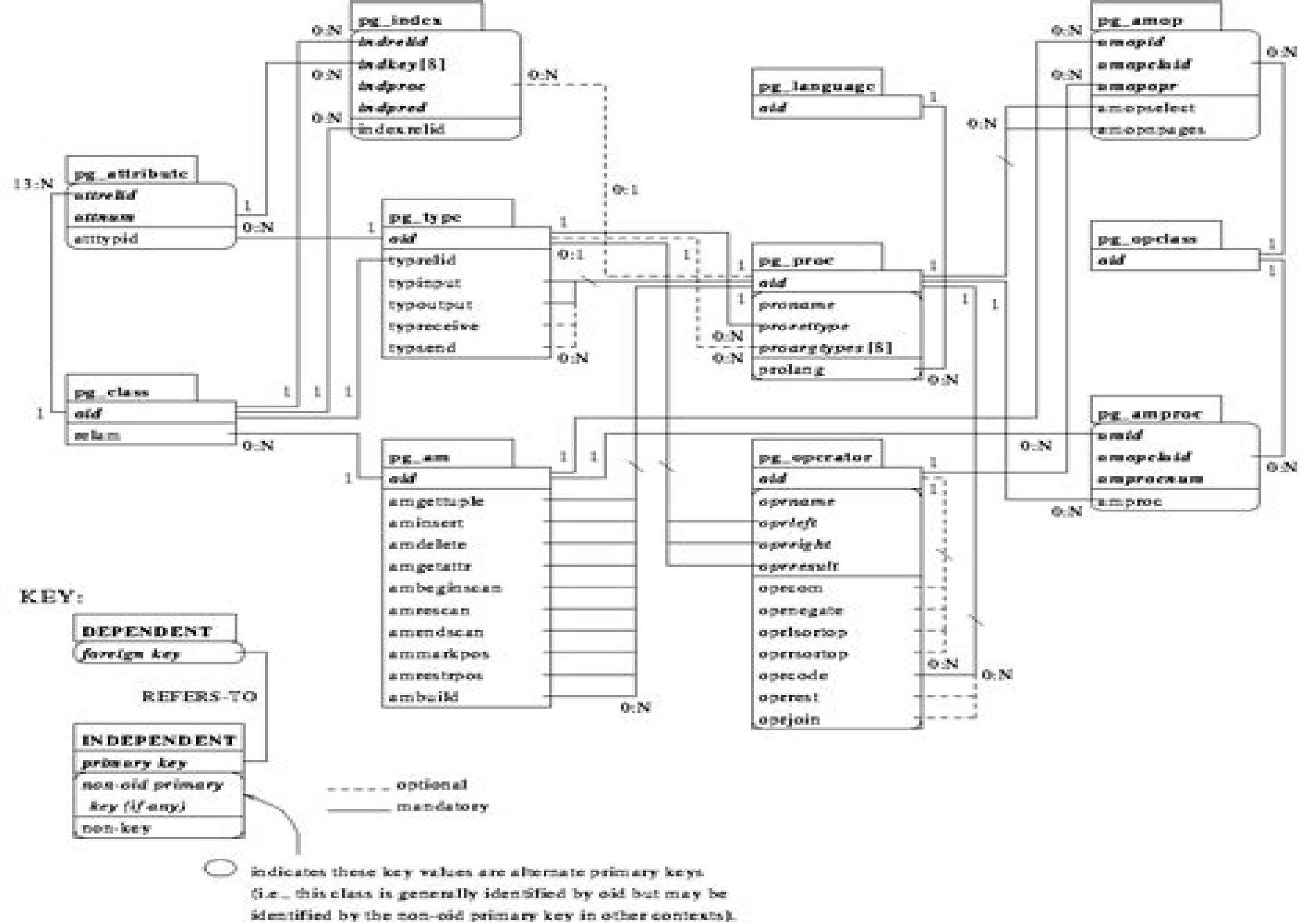
Figure 3. The major POSTGRES system catalogs.
