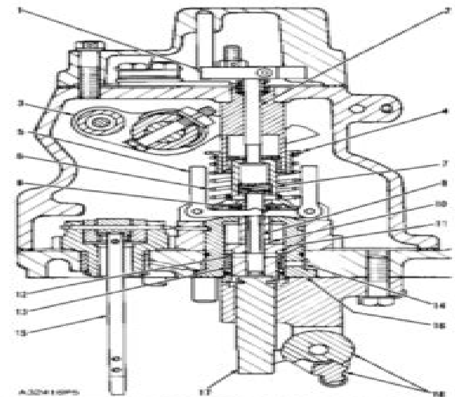
Hydra-Mechanical Governor For Standard Engines (Carter)
