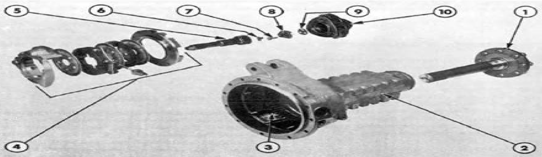
Figure 3 Rear Axle Assembly—Ford 5600, 6600 and 6700
