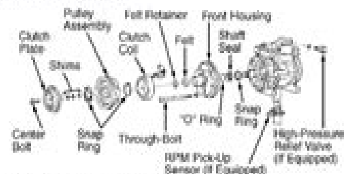
Fig. 3: Compressor (Nippondenso 10PA17C, 10PA15 & 10PA20 Are Similar) Courtesy of Mitsubishi Motor Sales of America
