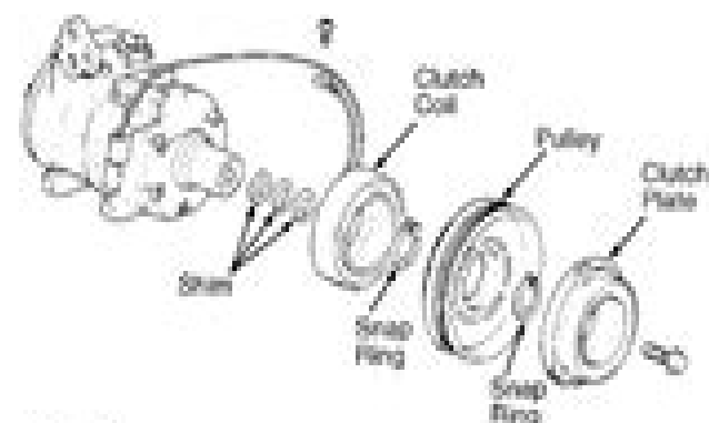
Fig. 2: Exploded View Of Compressor (Nippondenso 10PA17C 10-Cyl.) Courtesy of Toyota Motor Sales, U.S.A., Inc.
