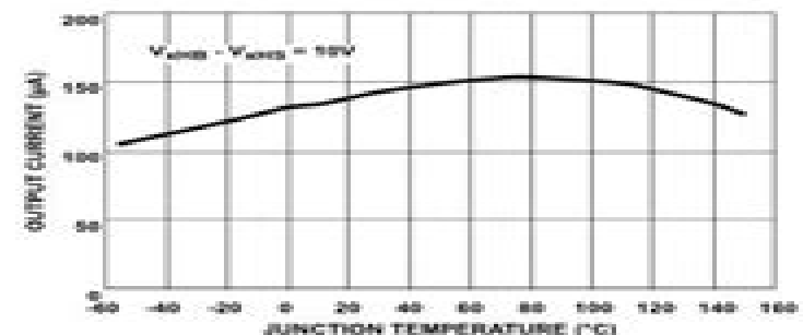
FIGURE 2. CHARGE PUMP OUTPUT CURRENT
