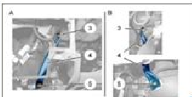
Figure 9: Removal of the oil filler cap.
