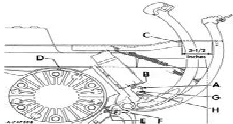
Illustr. 101 Brake pedal adjustment.
