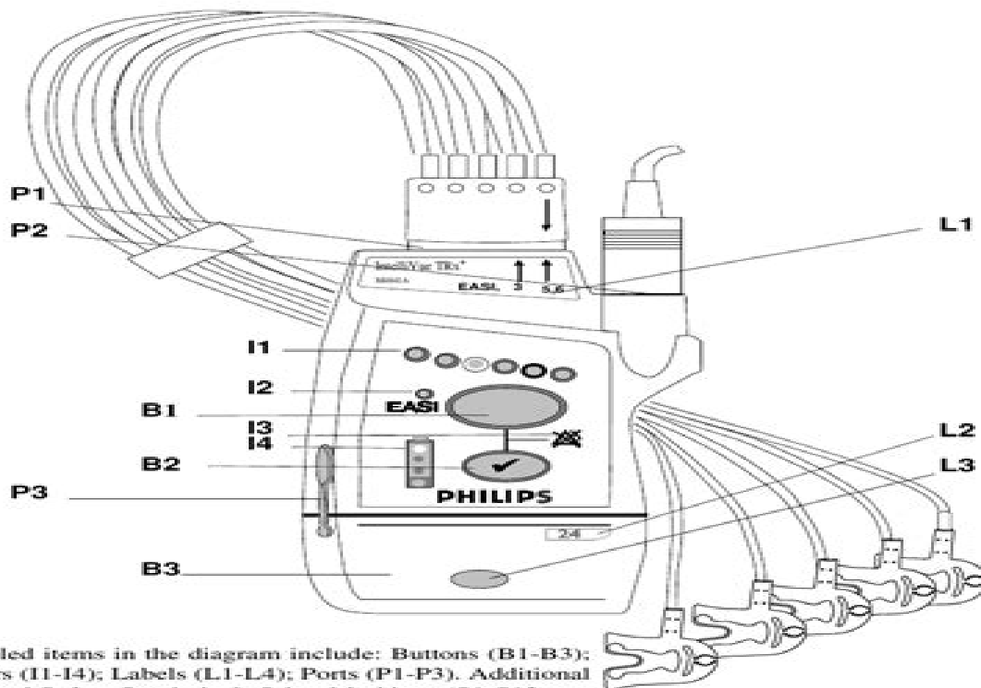
IntelliVue TRx+ Transceiver - Front View
